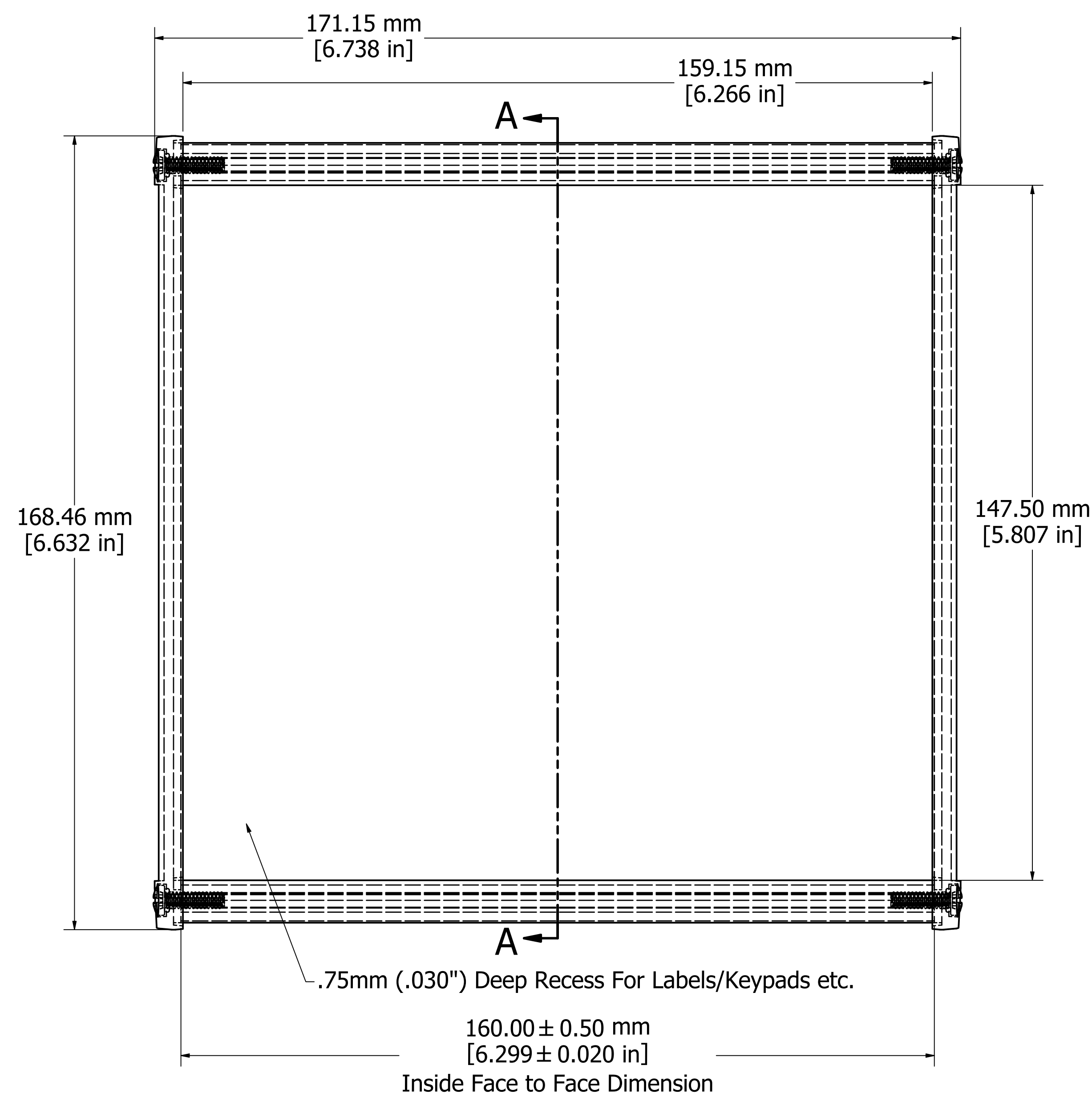
ASSEMBLY - TOP VIEW
