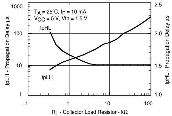
Figure 13. Propagation Delay vs. Collector Load Resistor
