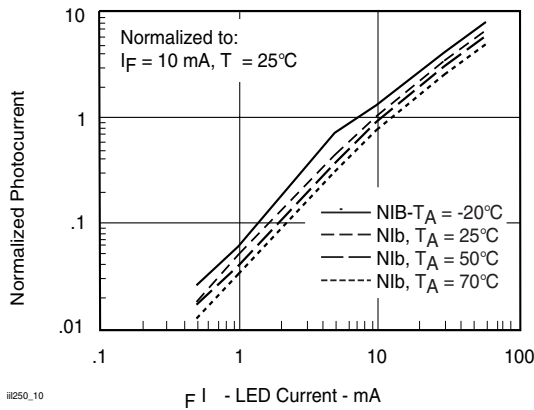
Figure 10. Normalized Photocurrent vs. I_F and Temp.
