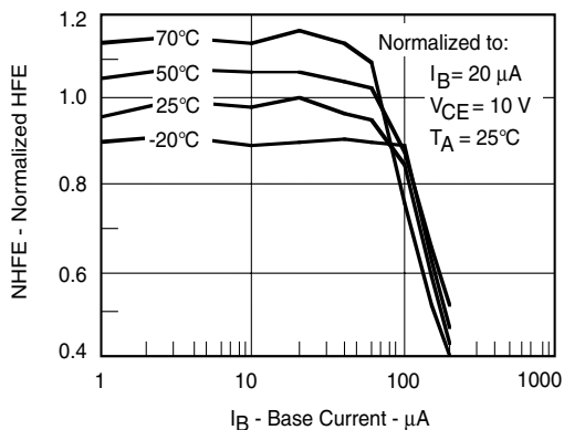
Figure 11. Normalized Non-saturated HFE vs. Base Current and Temperature
