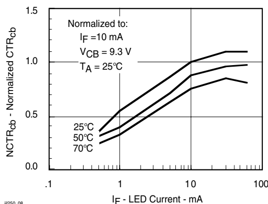
Figure 8. Normalized CTR_{cb} vs. LED Current and Temperature
