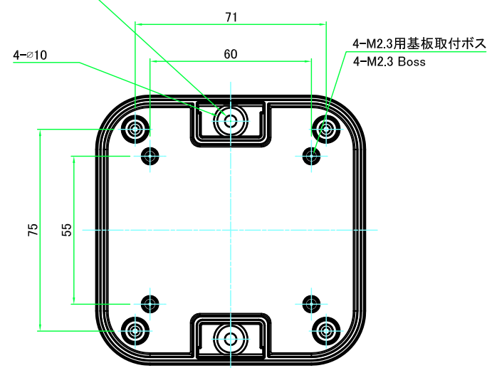
2-M4用外部取付穴 2-M4 Mounting hole
