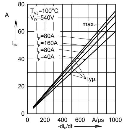
Fig. 3 Peak reverse current versus -di_F/dt .
