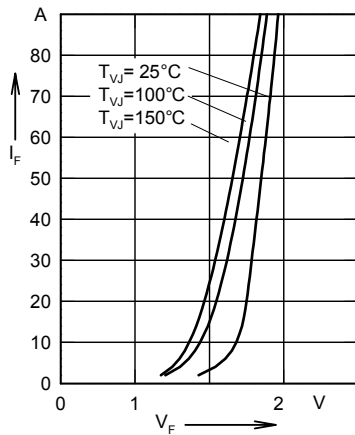
Fig. 1 Forward current versus voltage drop.
