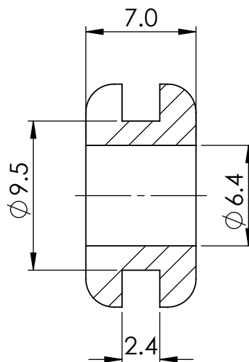
SECTION Y-Y
