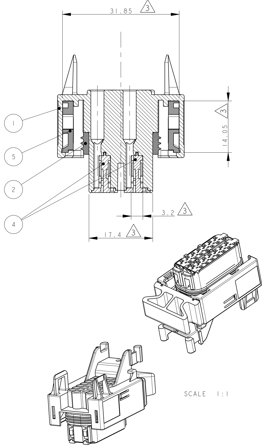
P/N 1393436-4 AS SHOWN (WAS SIEMENS No. V23542-C1028-B300)
