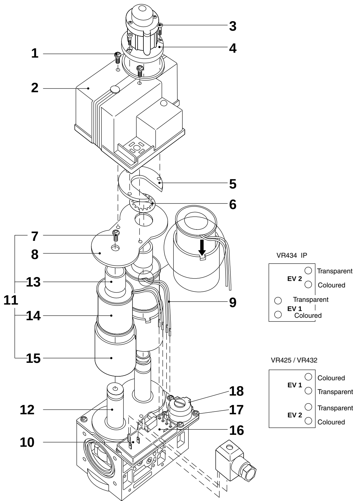
Fig. 20. Exploded view of the VR400/VR800 series
