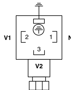
Fig. 8. Three pin electrical plug connector (according to ISO 4400) for IP applications.
