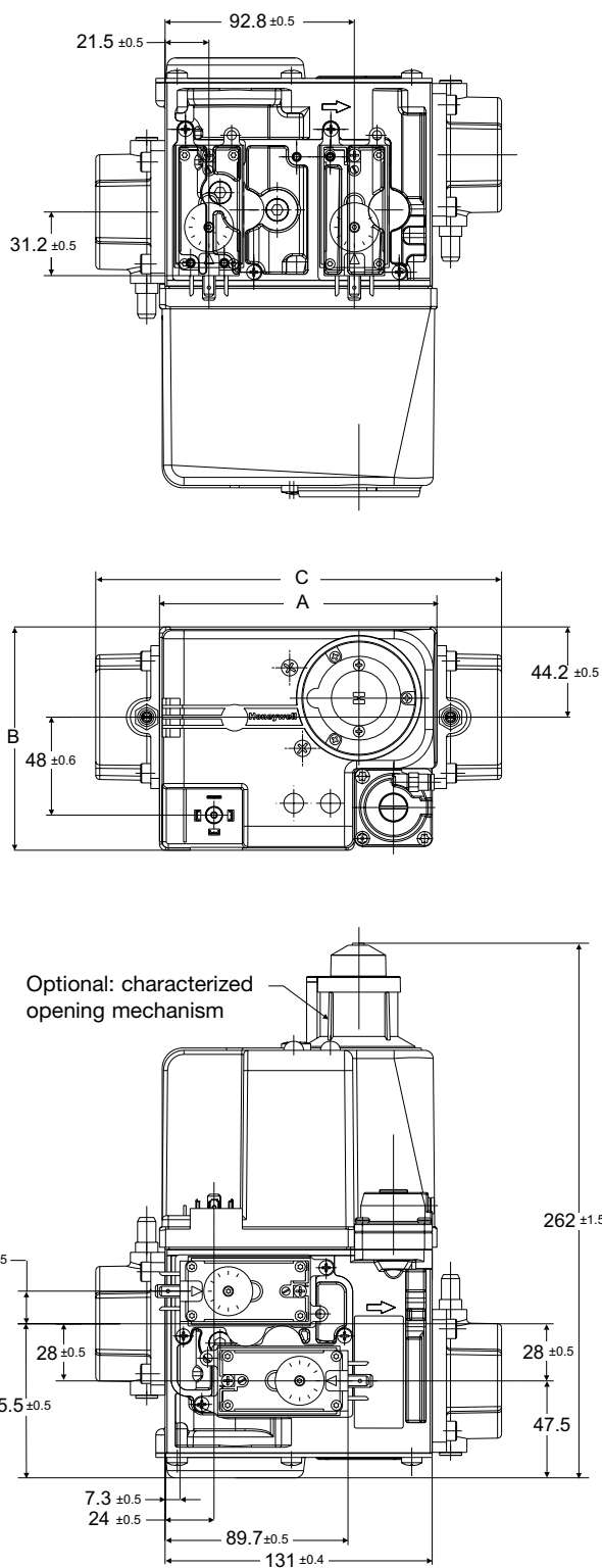
Fig. 6a. Dimensional drawing VR434/VR834 series (DN32)
