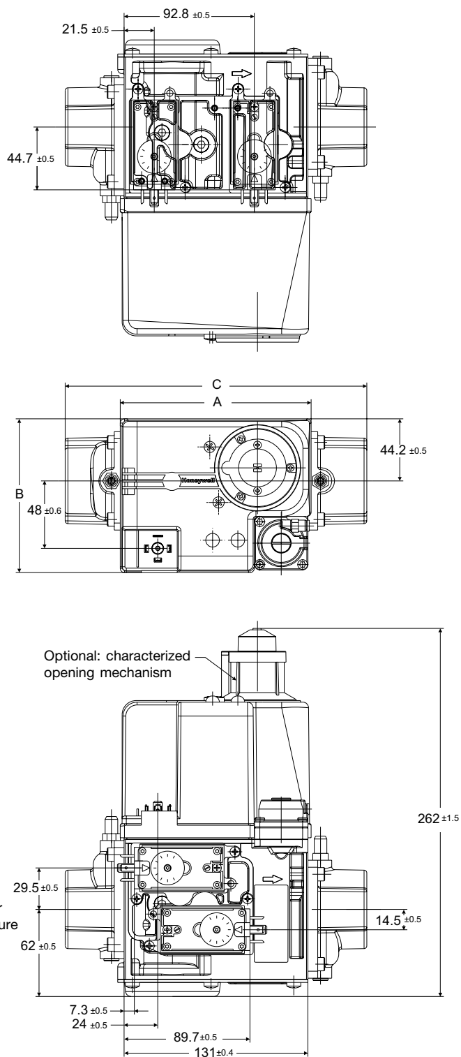
Fig. 7. Dimensional drawing VR434/VR834 series (DN32)
