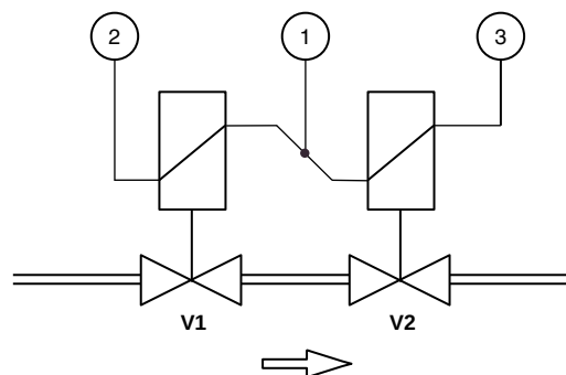
Fig. 10. Connection diagram VR400
