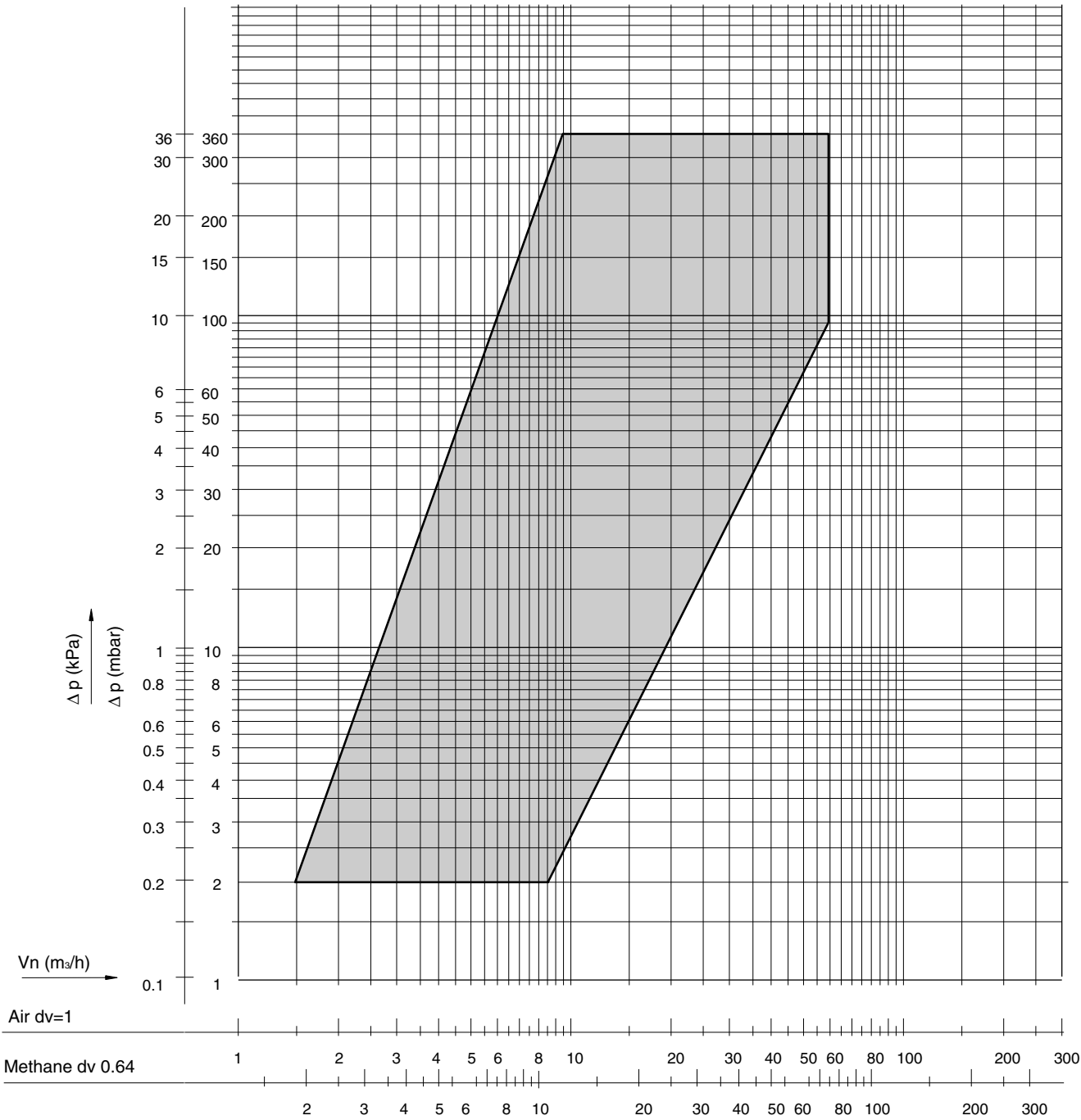
Fig. 3. Capacity curves for VR425/VR825 series (DN25)
