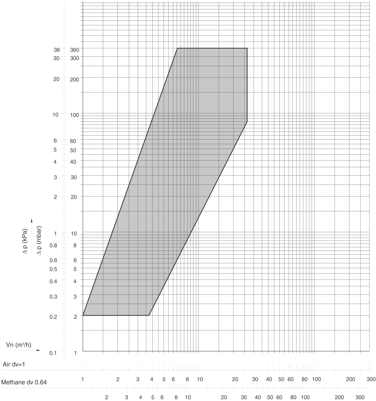
Fig. 1. Capacity curves for VR415/VR815 series (DN15)
