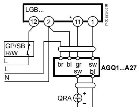
Connection diagram
