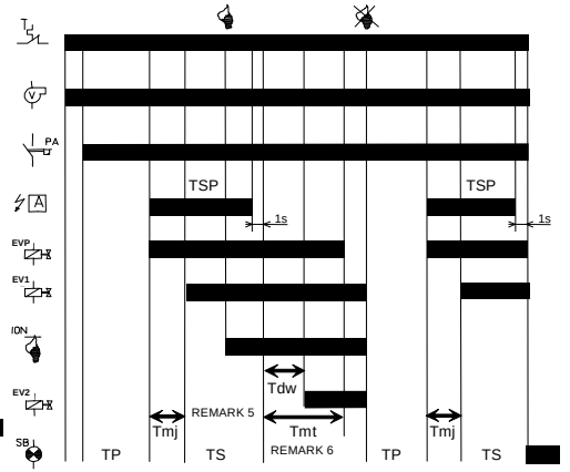
TGRD63 – TGRD83
