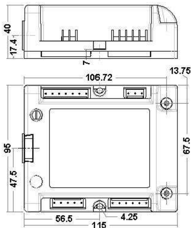
Fig. 1 – Overall dimensions
