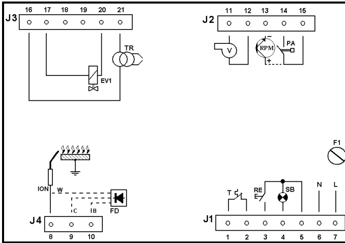
Type TGRD81
