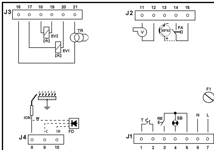
Type TGRD82
