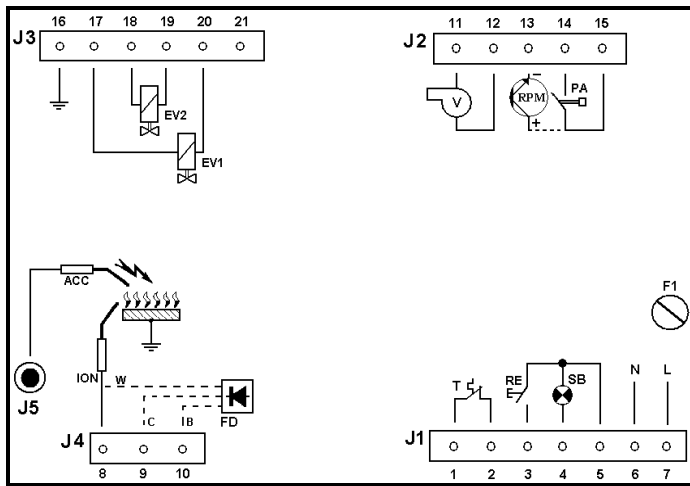
Type TGRD62
