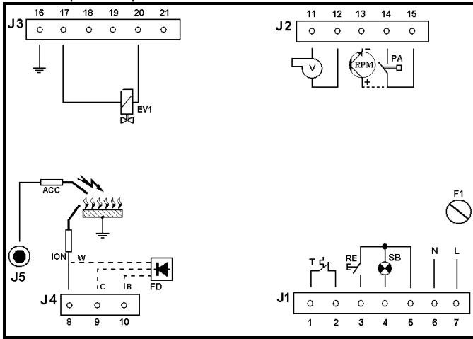
Type TGRD61
