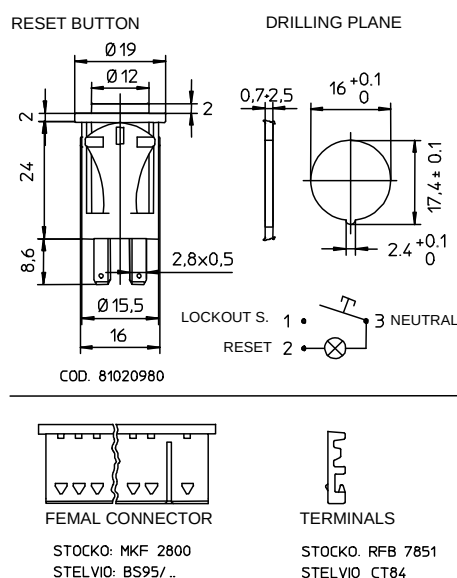
Fig. 2 – Standard accessories
