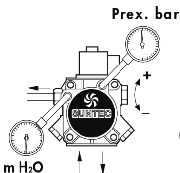
SUNTEC - AS 47
