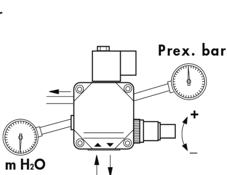
DANFOSS - BFP 11
