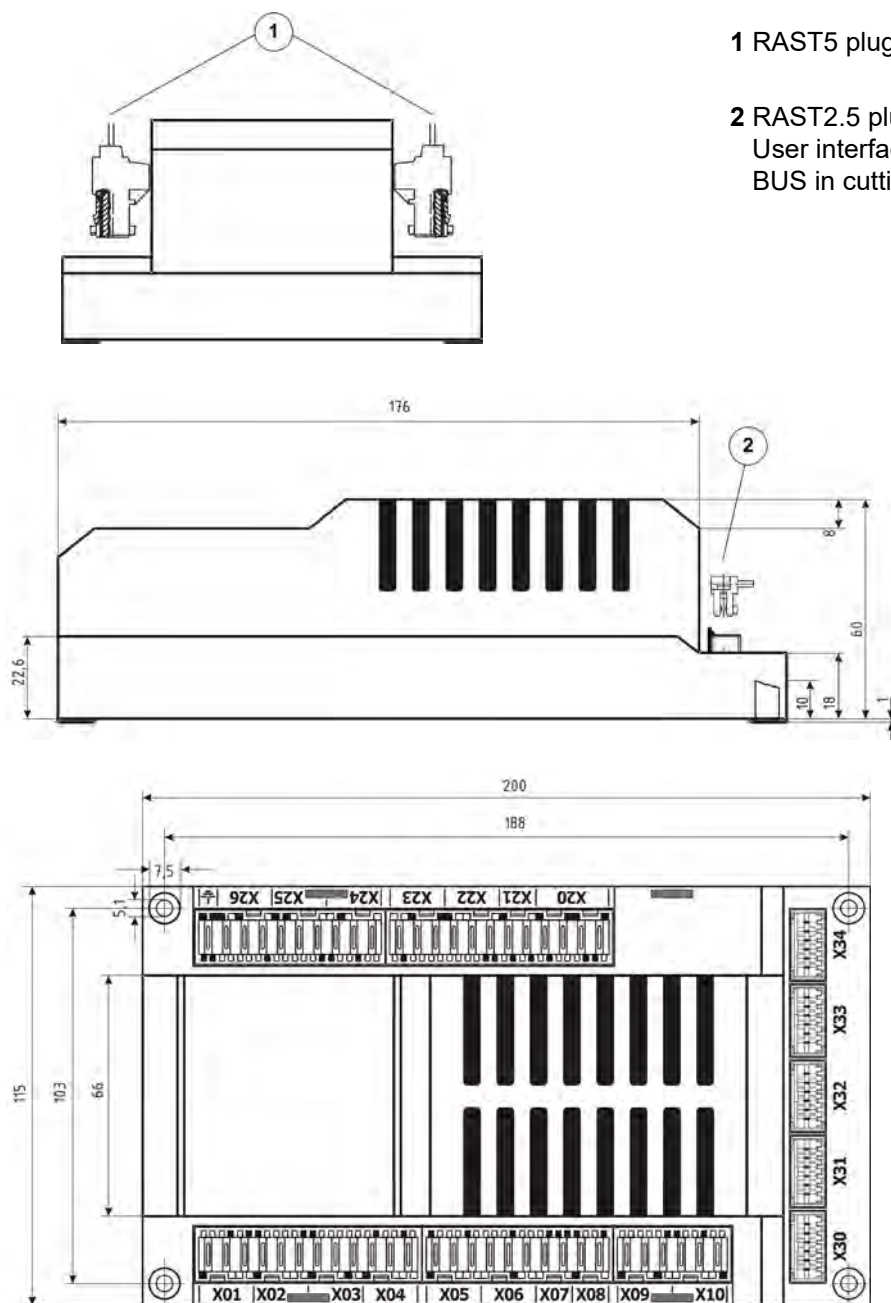
Fig. 2 Dimensions BT320 ... 341 (terminal assignment BT330/BT341 only)
