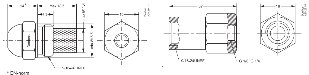
Nozzle holder
